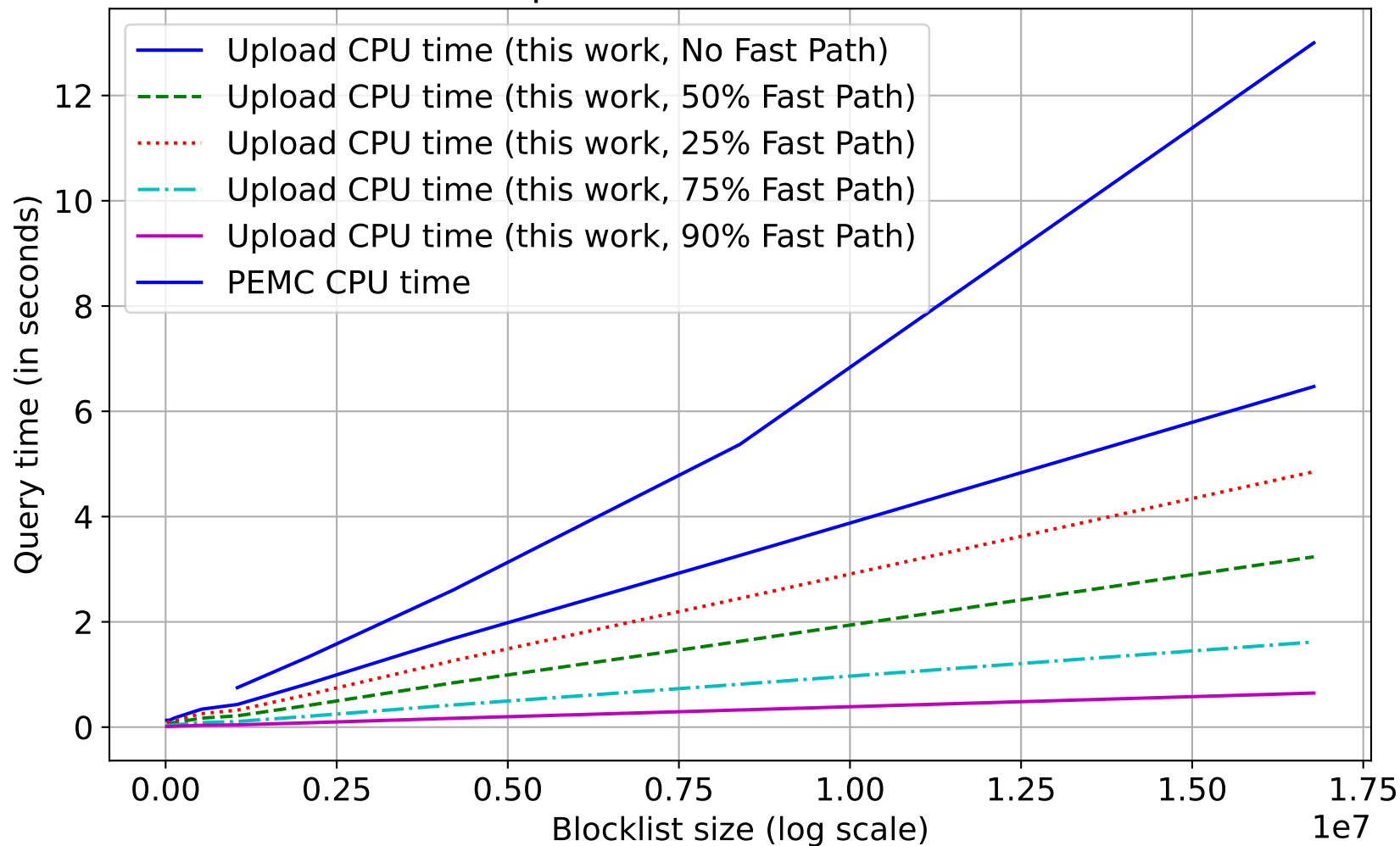
Compute time vs. Blocklist size
